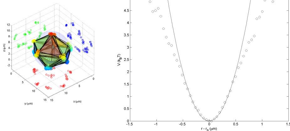
Figure 1: Left, superposition of 7 three-dimensional reconstructions of a droplet with 10 bound particles at time intervals of 0.033 seconds. Right, average potential of mean force between particles calculated from 200 consecutive 3D reconstruction; curve is best fit to a harmonic potential.
